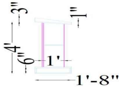
SIDE VIEW OF PODIUM SIZE (2'6"X1'8")
