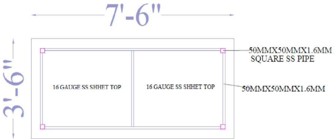
PLAN OF DINNING TABLE SIZE (7'6"X3'6")
